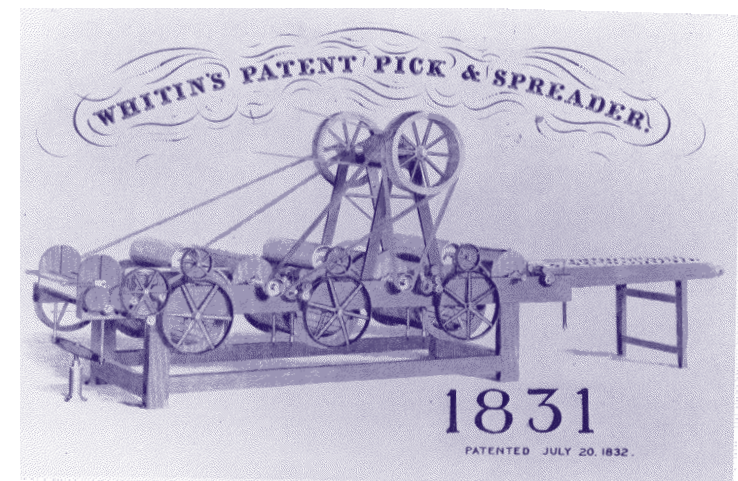
John Whitin excelled at making machinery to improve the production of cotton. This picker, which removed dirt and seeds from raw cotton, was his first product and the foundation of the family's subsequent dominance in the textile machinery field.
